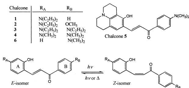
Scheme 1. Structures and photoisomerization of chalcones in neutral solution.
