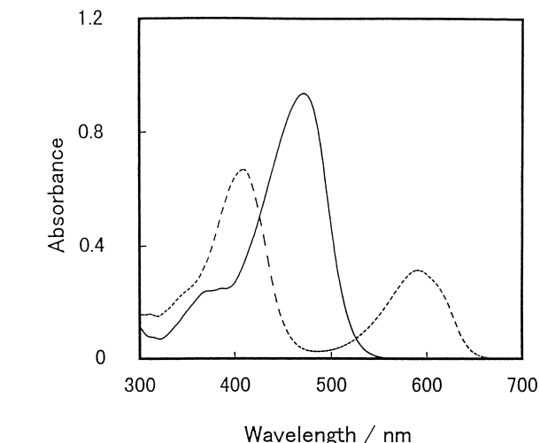
Fig. 4. Absorption spectra of the photoisomer (PSS solution) of chalcone 3 in toluene immediately after irradiation with 405 nm light (solid curve), and spectra after addition of 50 \mu\text{M} trifluoroacetic acid (broken curve). No such spectral change was observed by addition of the acid to the solution before irradiation.
