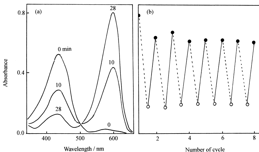
Fig. 5. Photochromism of chalcone 4 (10 \mu\text{M} ) in a 1:1 aqueous ethanol solution at pH 6.0. (a) Photochemical conversion into flavylium ion on irradiation with 405 and 436 nm beams from a 400-W high-pressure mercury lamp. (b) Photochromic reversibility toward repeated cycles of photocoloration for 25 nm (solid lines) and thermal reversion on heating at 60 ^{\circ}\text{C} for 100 min (broken lines).
