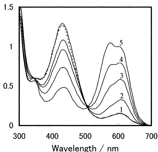
Fig. 6. Photochemical conversion of chalcone 3 (5 wt%) into flavylium ion in PMMA film in the presence of 10 wt% tannic acid, on irradiation with 405 and 436 nm beams from a 120-W high-pressure mercury lamp. Irradiation time/min: (1) 0, (2) 10, (3) 30, (4) 60, and (5) 120, respectively. Broken curve refers to the thermal change on standing at room temperature for 24 h.
