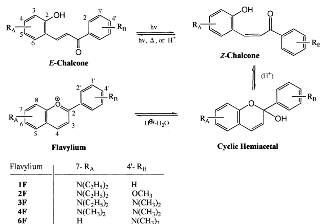
Scheme 2. Interconversions among E/Z -isomers of chalcones and flavylium ions.
