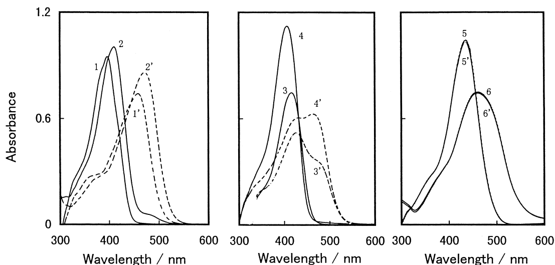
Fig. 2. Photochemical isomerization of chalcone 3 in hexane (1,1'), toluene (2,2'), acetone (3,3'), ethyl acetate (4,4'), ethanol (5,5'), and water (6,6'). Solid curves: before irradiation, broken curves: after irradiation with sunlight for one minute. Each solution contained 8.5% of 1,2-dimethoxyethane.
