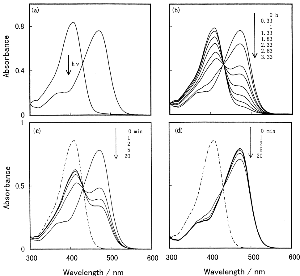
Fig. 1. Photochemical isomerization of chalcone 3 in toluene solution (30 \mu\text{M} ) on irradiation with 405 nm light for one minute (a), followed by thermal reversion at 30 °C (b), and photochemical reversion with light of \lambda > 460 nm 4 °C (c) where thermal reversion is substantially depressed (d).
