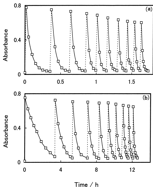
Fig. 3. Reversibility toward the repeated cycles for the photochemical isomerization (broken curves) and thermal reversion (solid curves) of chalcones 1 (a) and 2 (b) in toluene solution at 30 °C. The vertical axes refers to the absorbance of the photoisomers.
